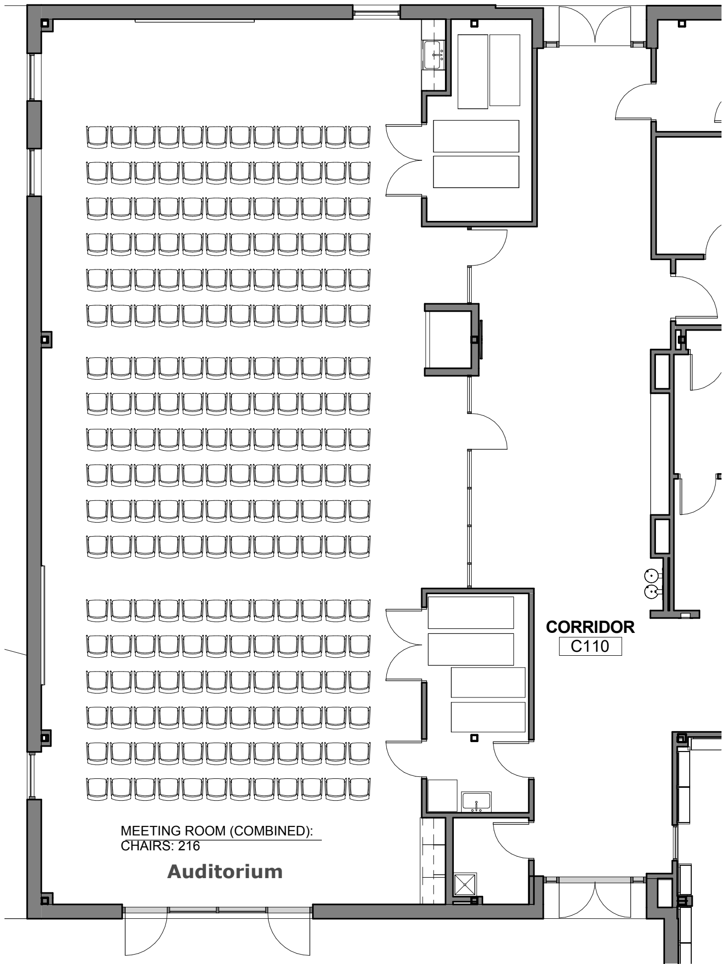
1 PARTIAL PLAN - MEETING ROOMS LECTURE CHAIRS - COMBINED P0.00 1/8" = 1'-0"
