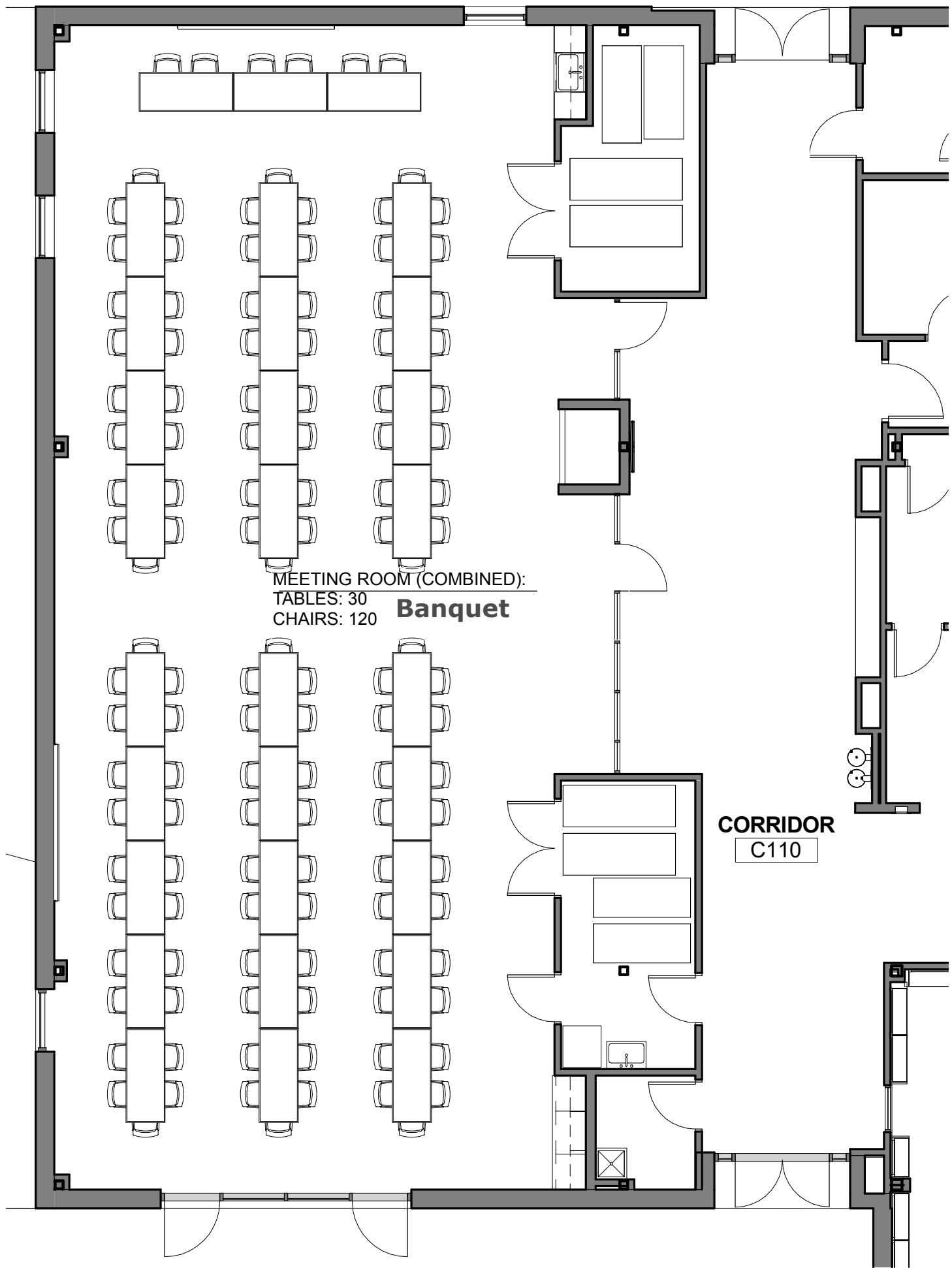
1 PARTIAL PLAN - MEETING ROOMS BANQUET (ROWS) - COMBINED P0.00 1/8" = 1'-0"
