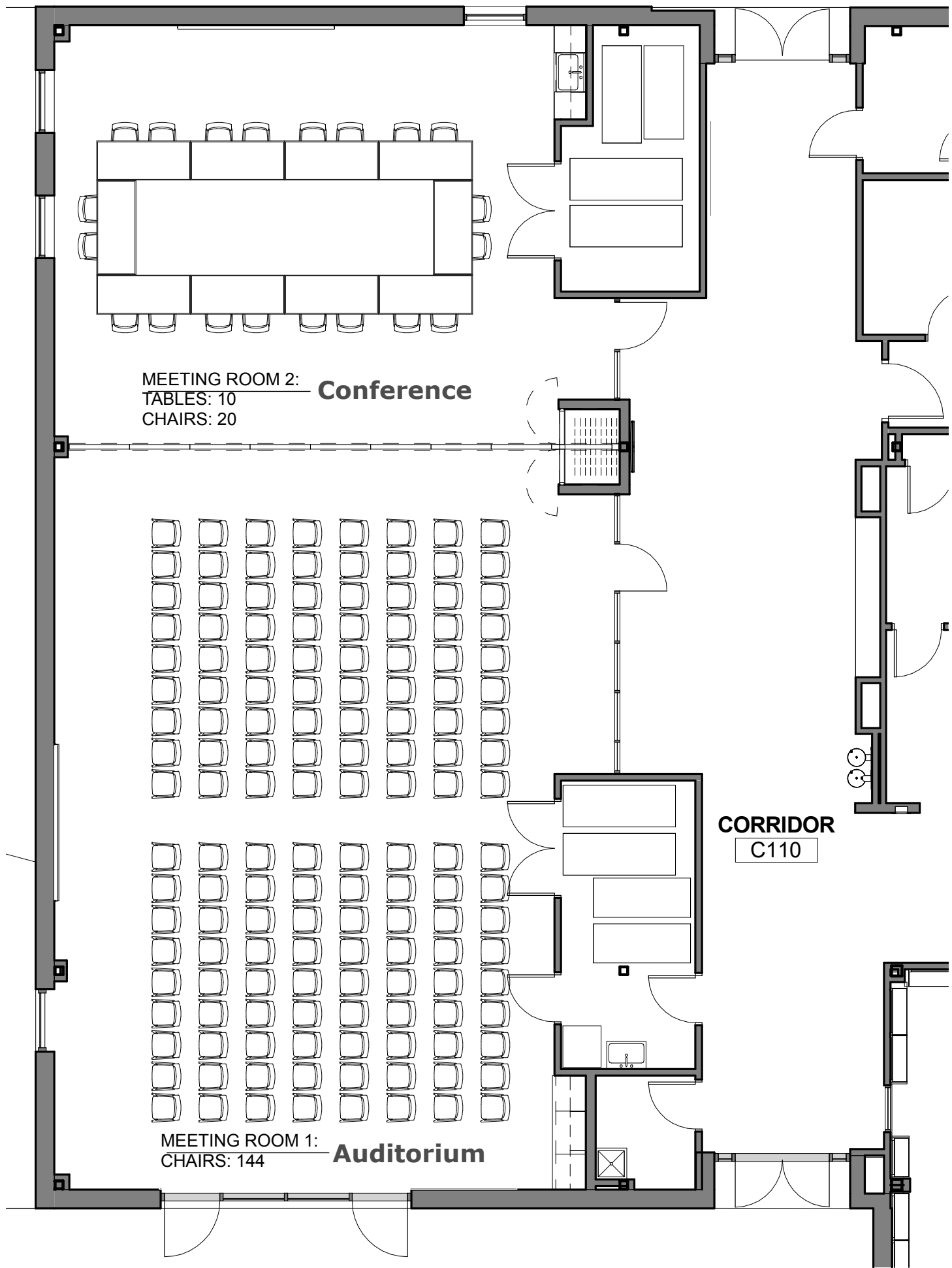
1 PARTIAL PLAN - MEETING ROOMS MIXED USE - DIVIDED P0.00 1/8" = 1'-0"
