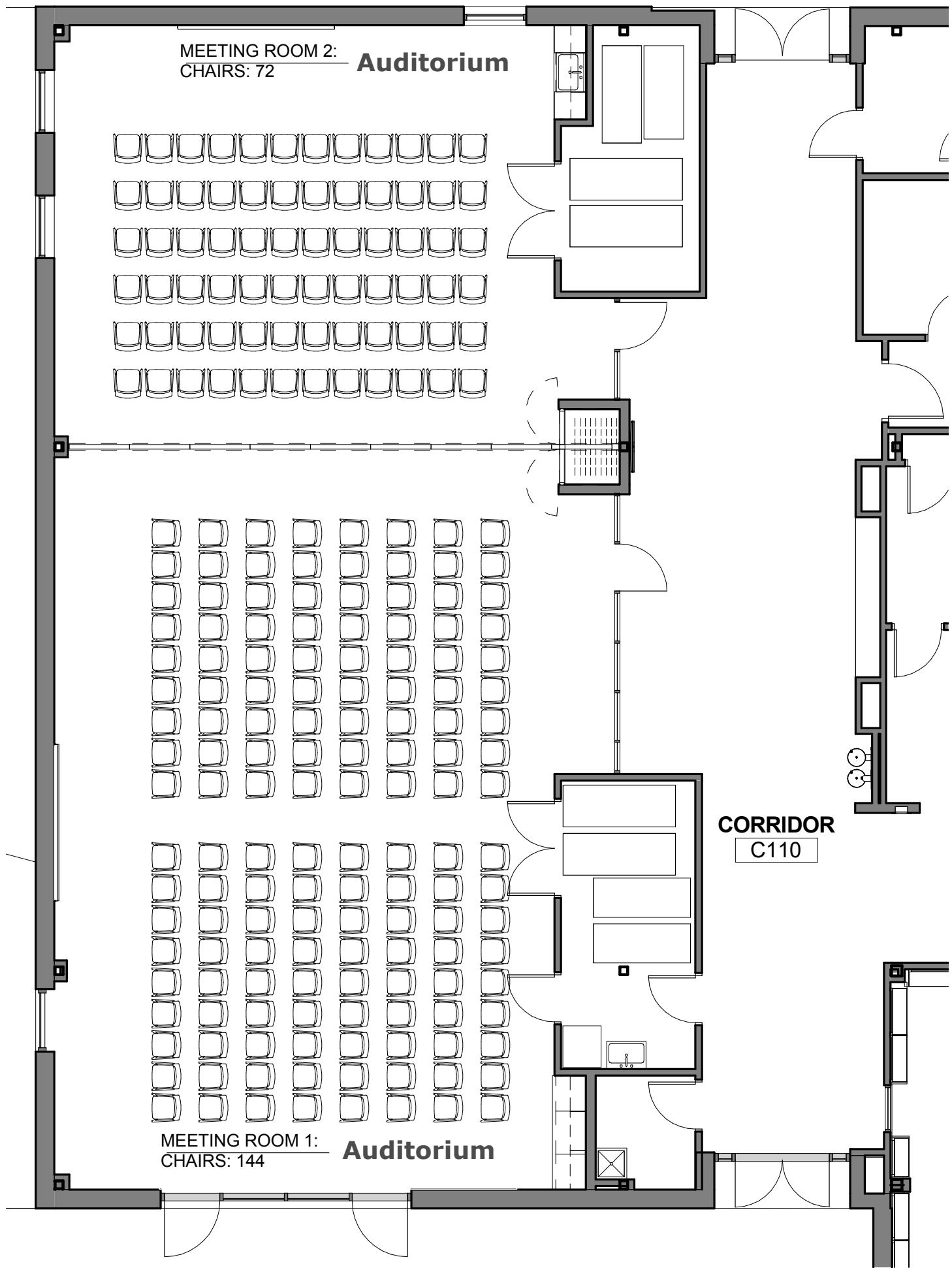
1 PARTIAL PLAN - MEETING ROOMS LECTURE CHAIRS - DIVIDED P0.00 1/8" = 1'-0"
